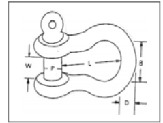
ANCHOR Screw Pin Shackle
